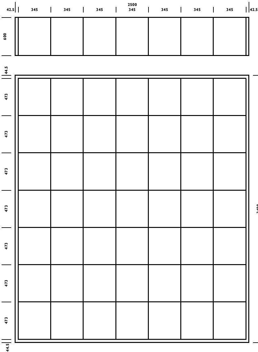
MDF PLATES EGGER U727 MDF 15MM - BACK
